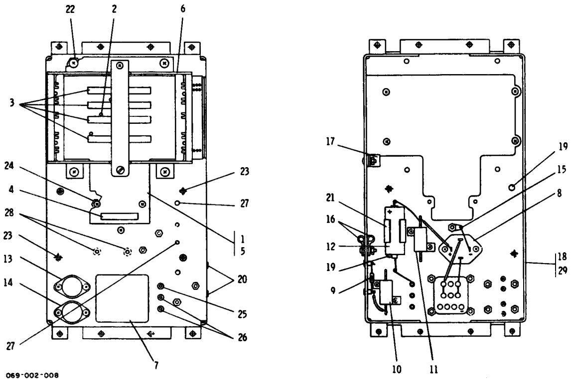
Figure 6-8. Chassis Assembly
