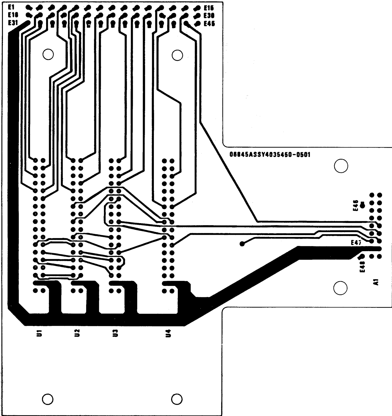
Figure 3-7. Motherboard, Track Wiring, Schematic Diagram (Sheet 1 of 2)
