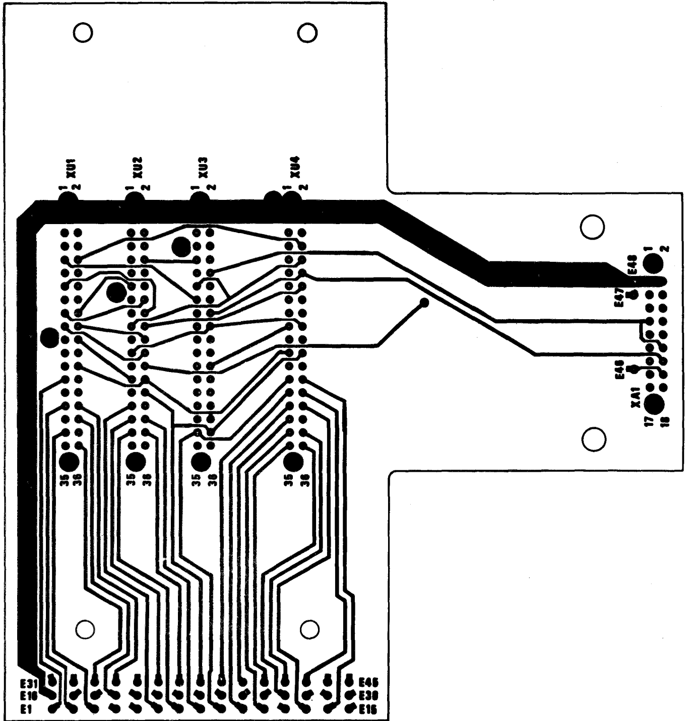
Figure 3-7. Motherboards, Track Wiring, Schematic Diagram (Sheet 2 of 2)
