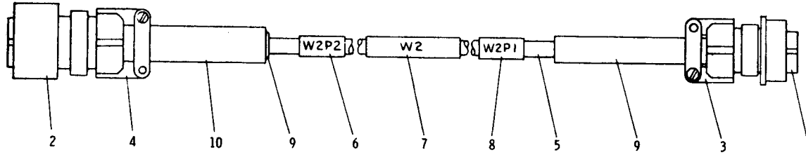
Figure 6-5. Power Cable Assembly (PN 4035549-0501)
