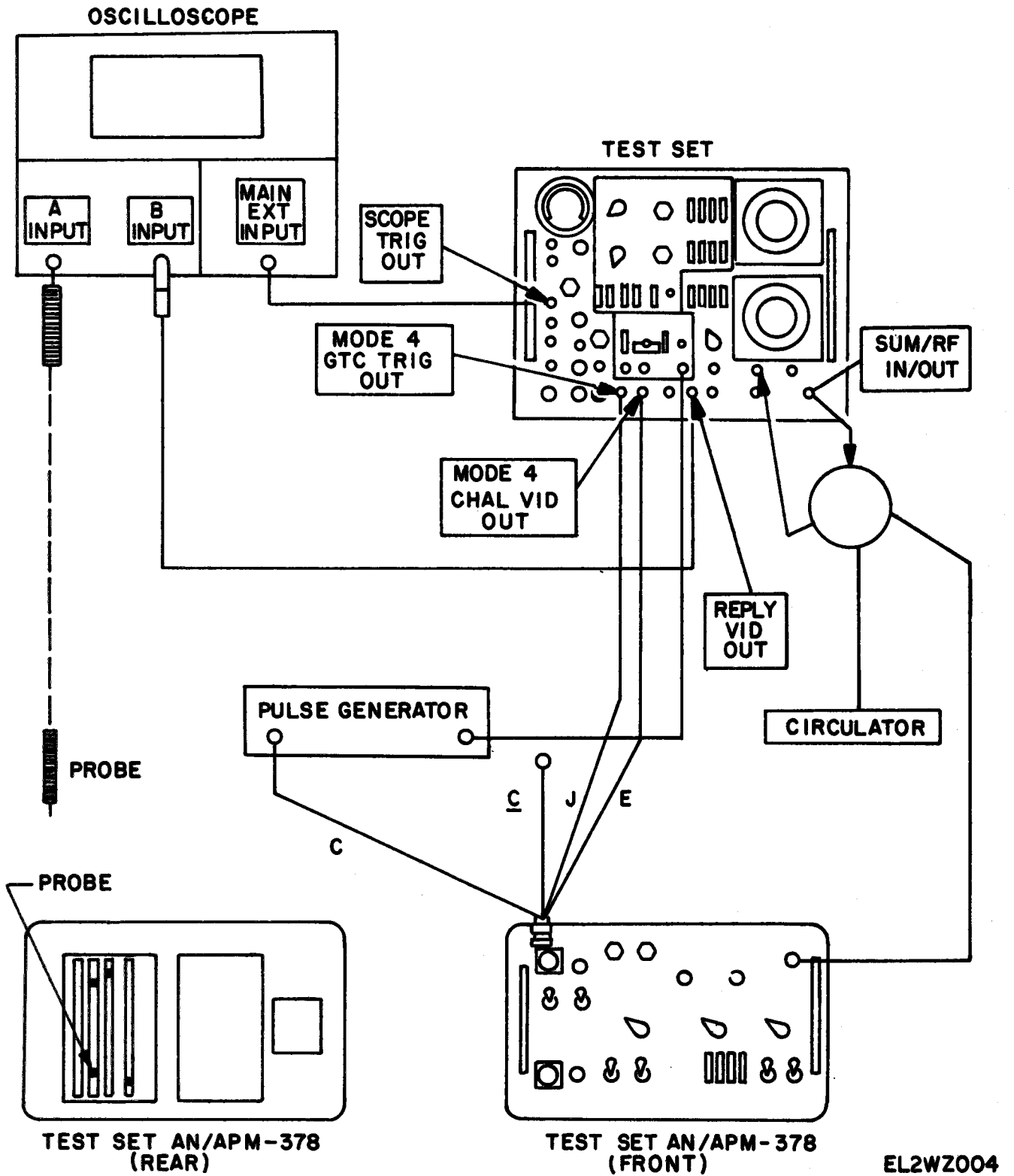
FIGURE 4-4. MODE 4 TYPICAL TEST SETUP CONNECTIONS
