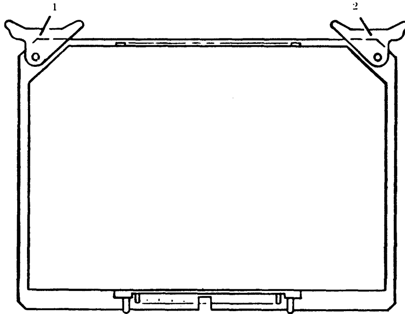
Figure 6-10. Module Assemblies
